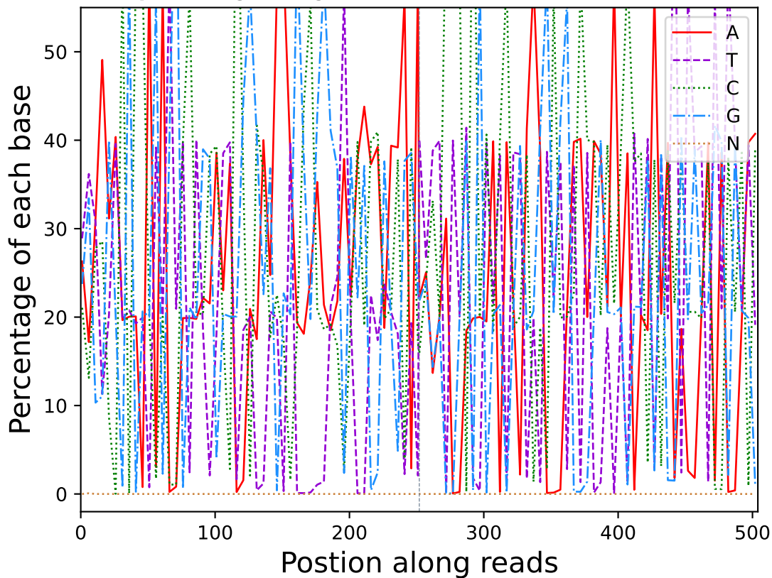
Base percentage along reads (R20107)
